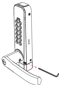
1. Remove grub screw
