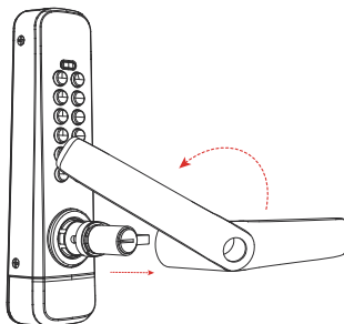
2. Remove handle, rotate to desired direction and replace onto lock body.
