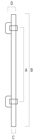
A 245mm B 400mm C 32x32mm D 65mm
