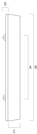
3942 - 300mm | 3944 - 600mm Pair back-to-back Blackbutt Hardwood
