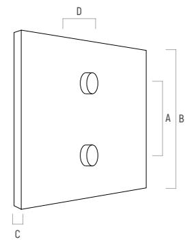
43932 Pair back-to-back Tempered Clear Glass
