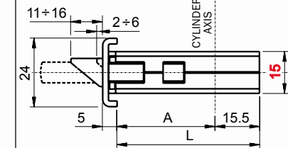
Lock "U" faceplate 24 X 5
