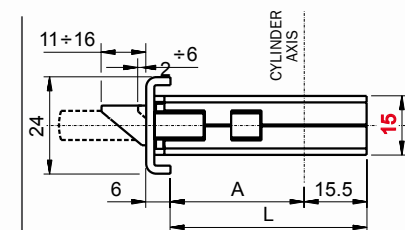
Lock "U" faceplate 24 X 6
