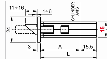
Lock flat faceplate 24 X 3
