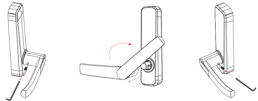
1. Remove grub screw
